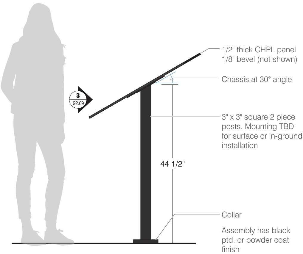
2 ST-15 - SIDE VIEW DETAIL G2.09 Scale: 3/4" = 1'-0"
